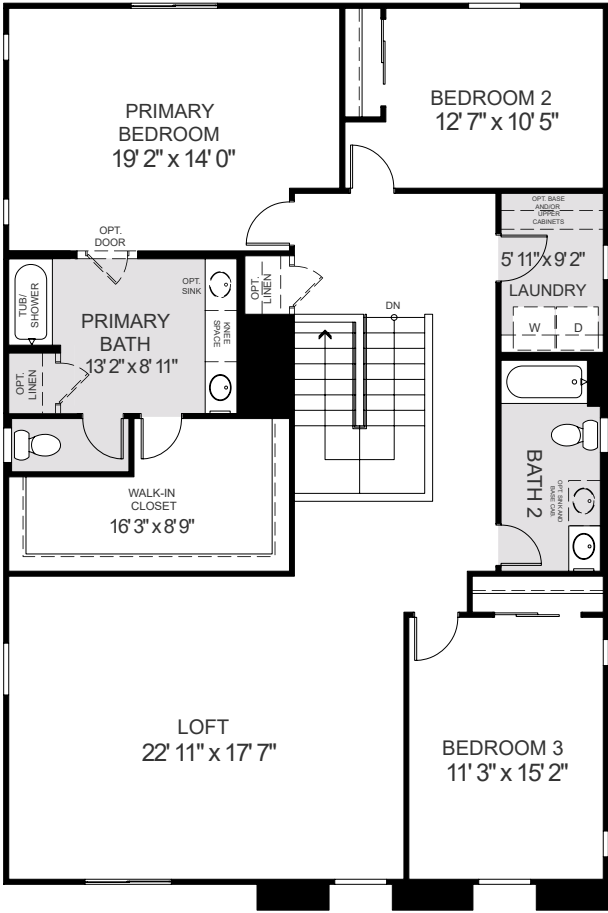
SECOND FLOOR
