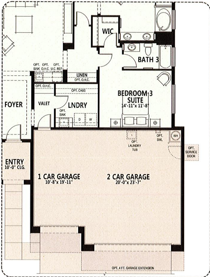
Opt. 3 Car Garage w/ Opt. Bedroom 3 Suite
